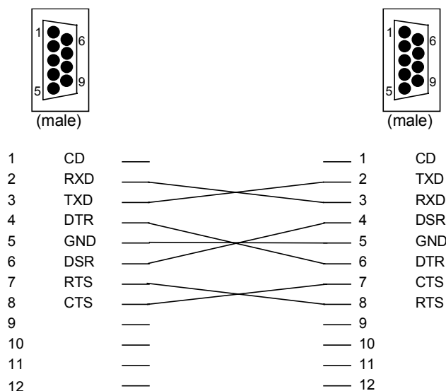
Fig. 14 Wiring of the adapter plug
