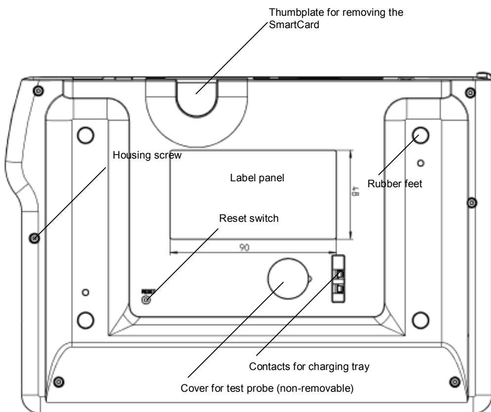
Fig. 2 Back of housing
