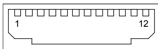
Fig. 3 Universal interface: "Lumberg" plug with pin numbering
