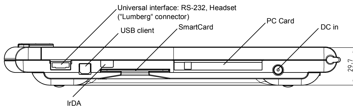
Fig. 1 Top edge with interfaces
