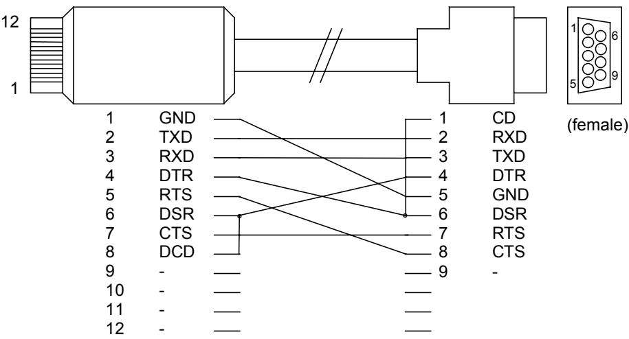
Fig. 13 Wiring of the serial connecting cable: SIMpad SL4 - PC
