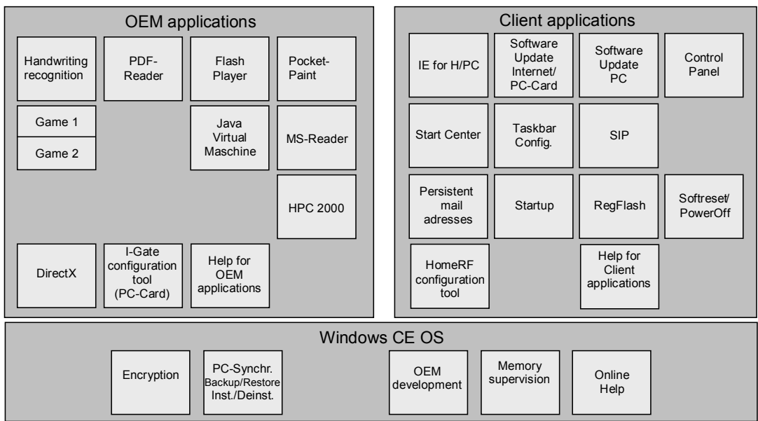
Fig. 4 File structure
