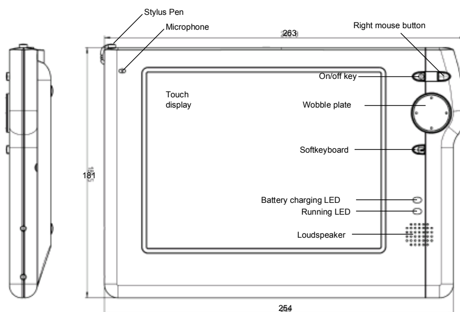
Fig. 1 Device design and controls
