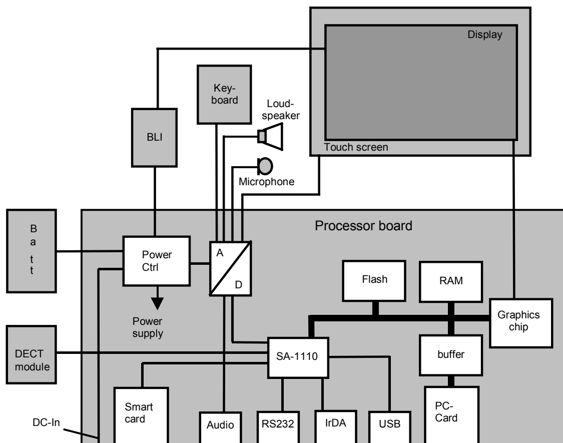
Fig. 3 SIMpad SL4 block diagram
